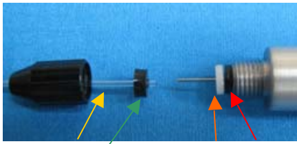
GLASS COMPRESSION ORING WHITE SPACER SEALING ORING
